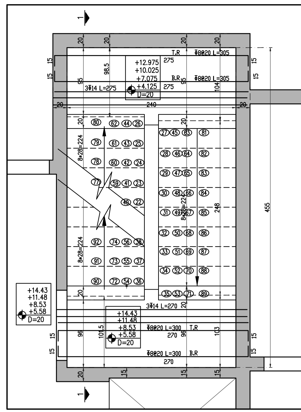
PLAN +5.58, +8.53, +11.48, +14.43
