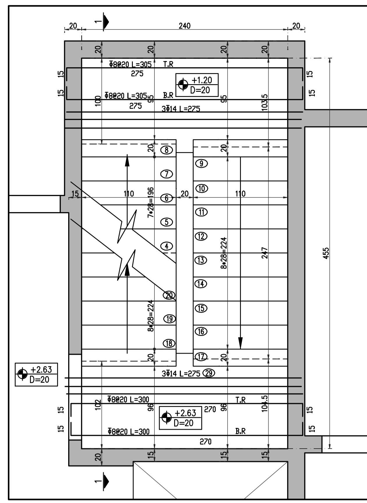
PLAN +2.63
