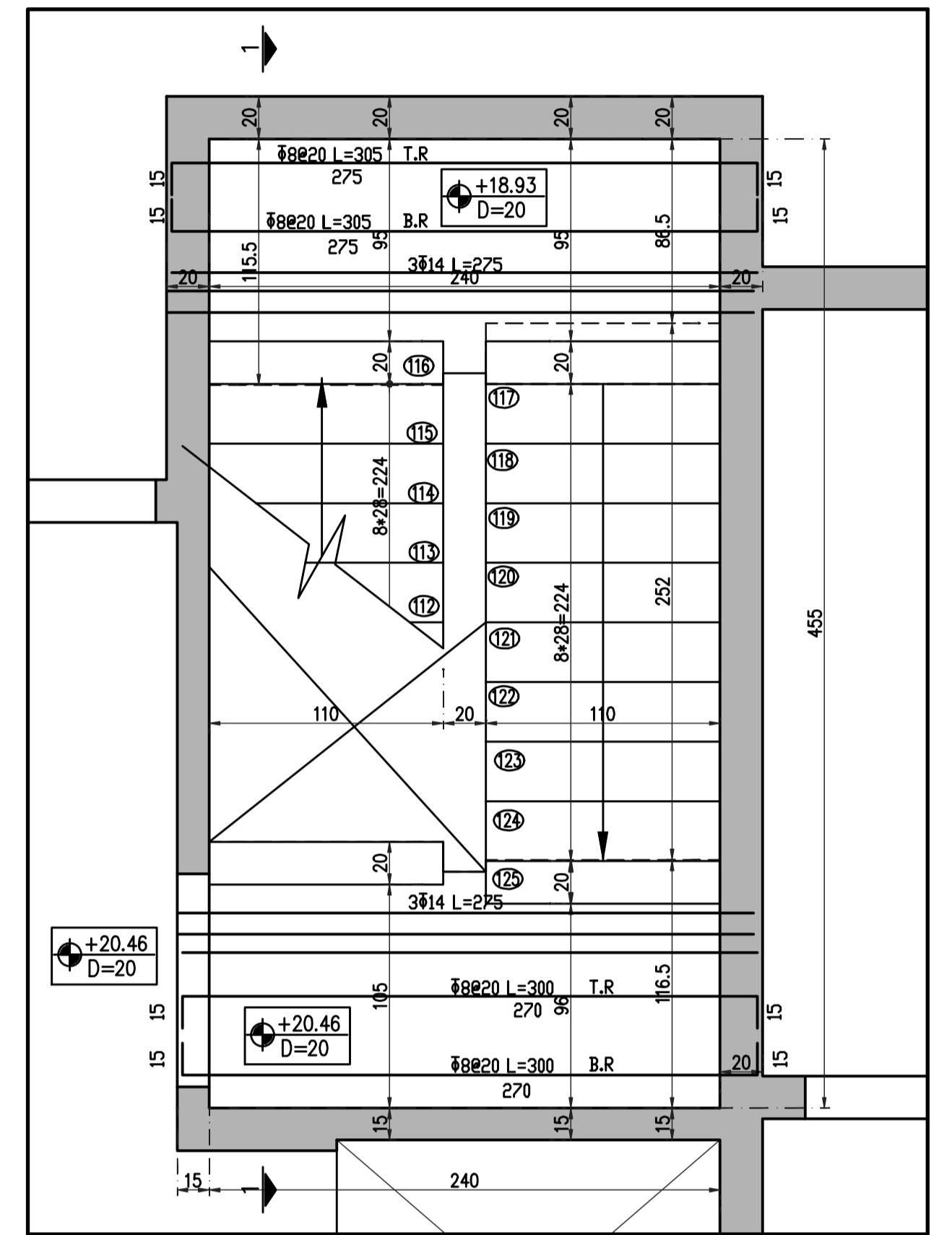
PLAN +20.46
