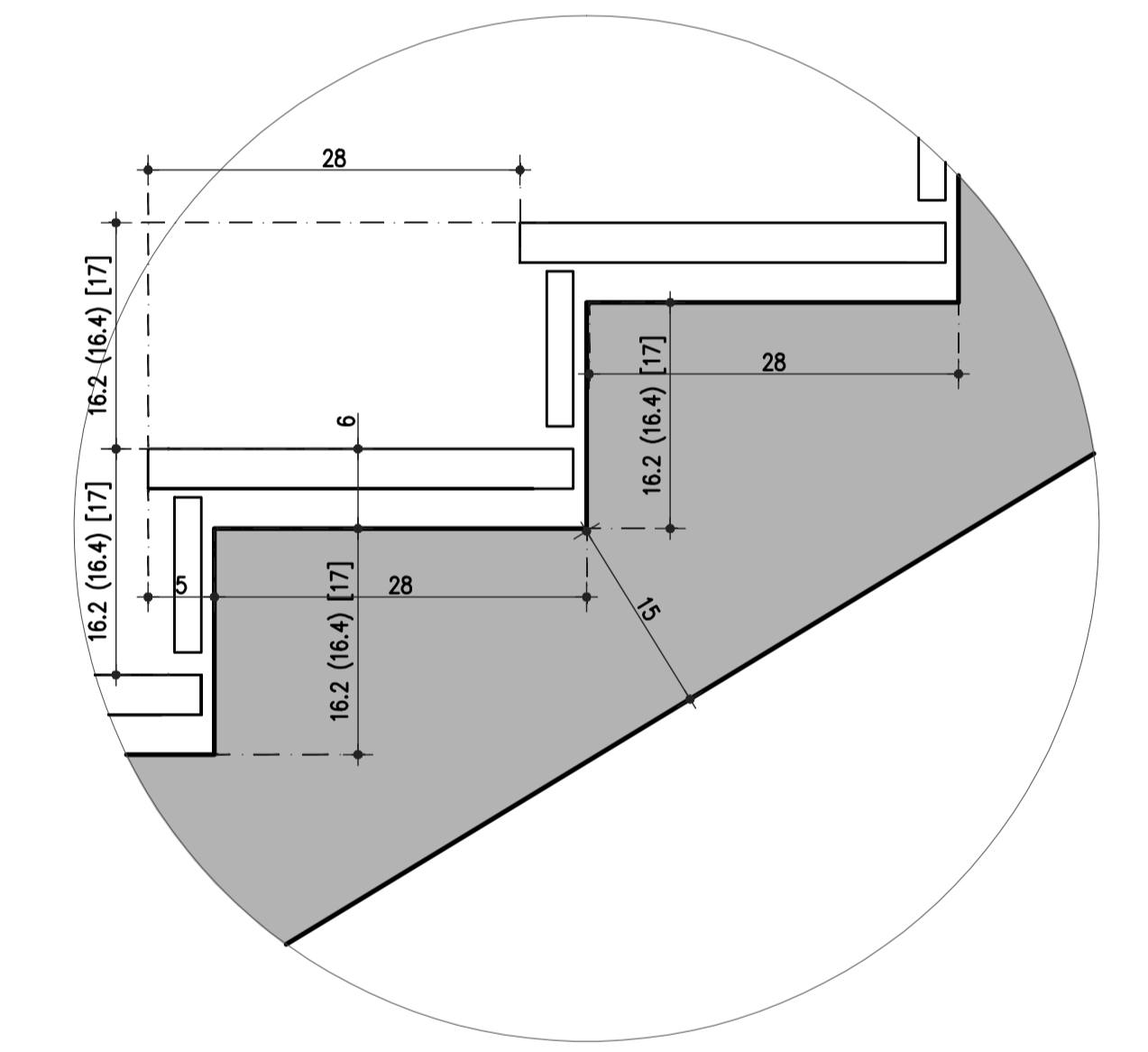
STAIR DETAIL
