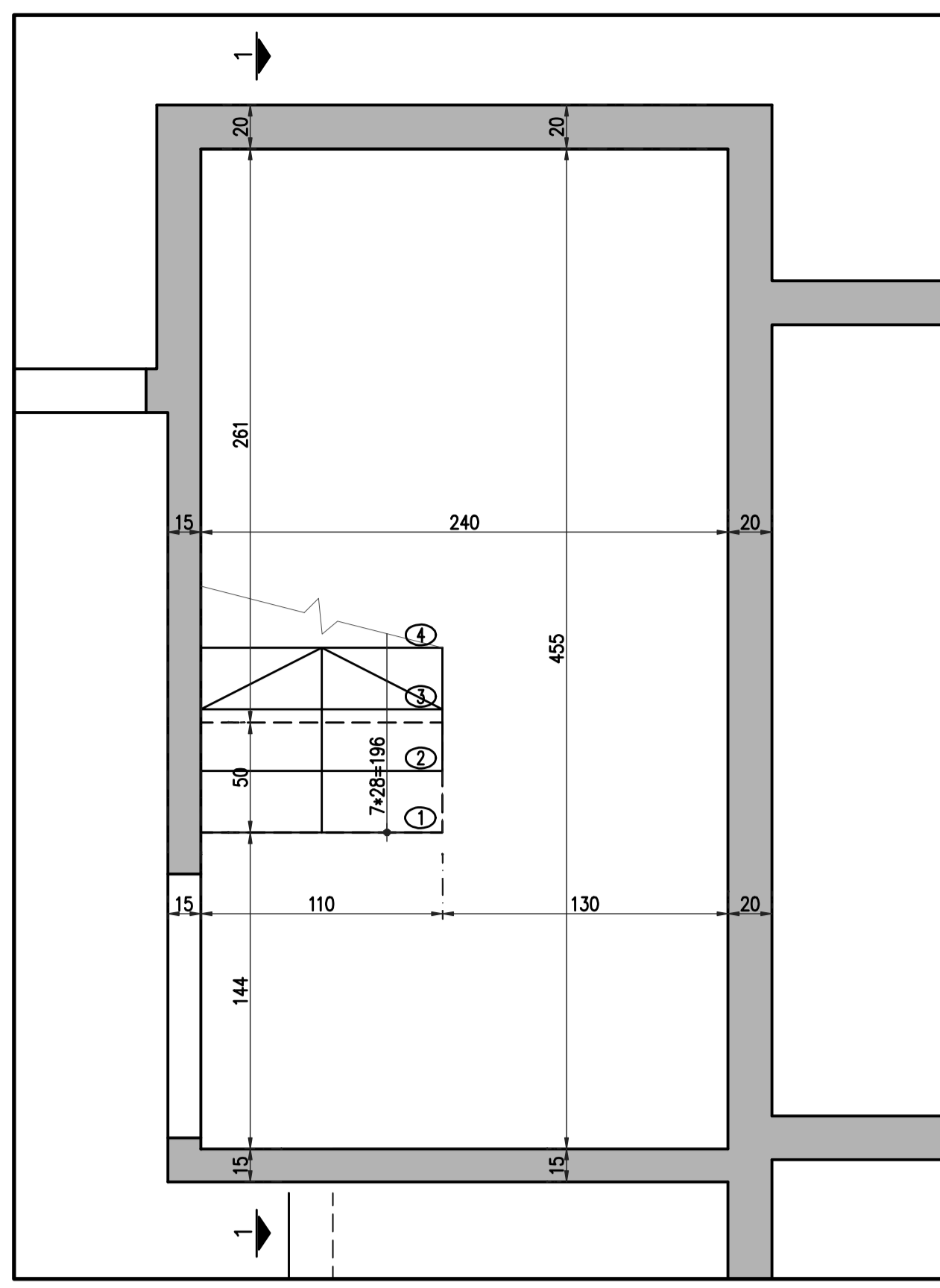
PLAN -0.12
