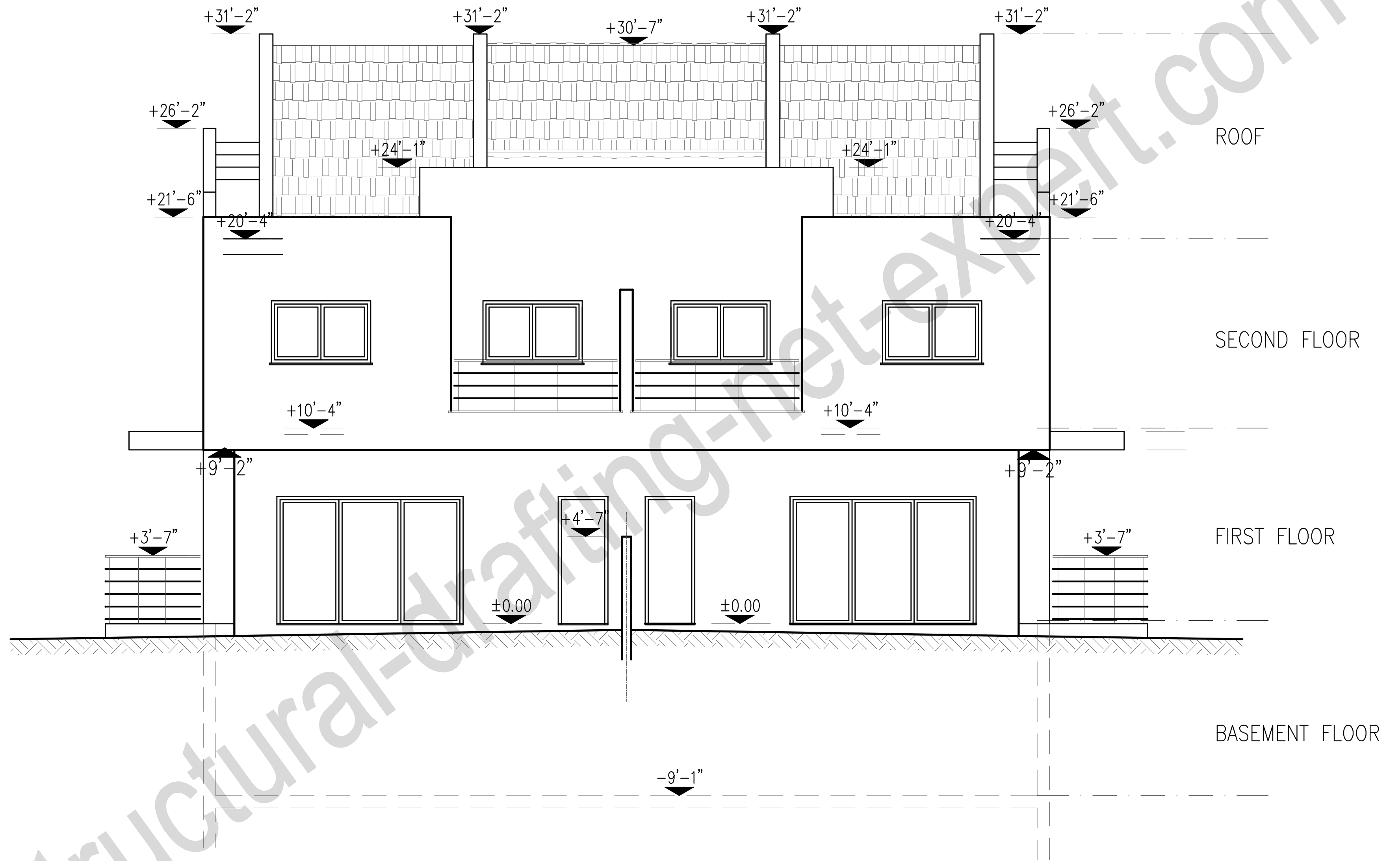
WEST SIDE ELEVATION SCALE 1/4" = 1'-0"
